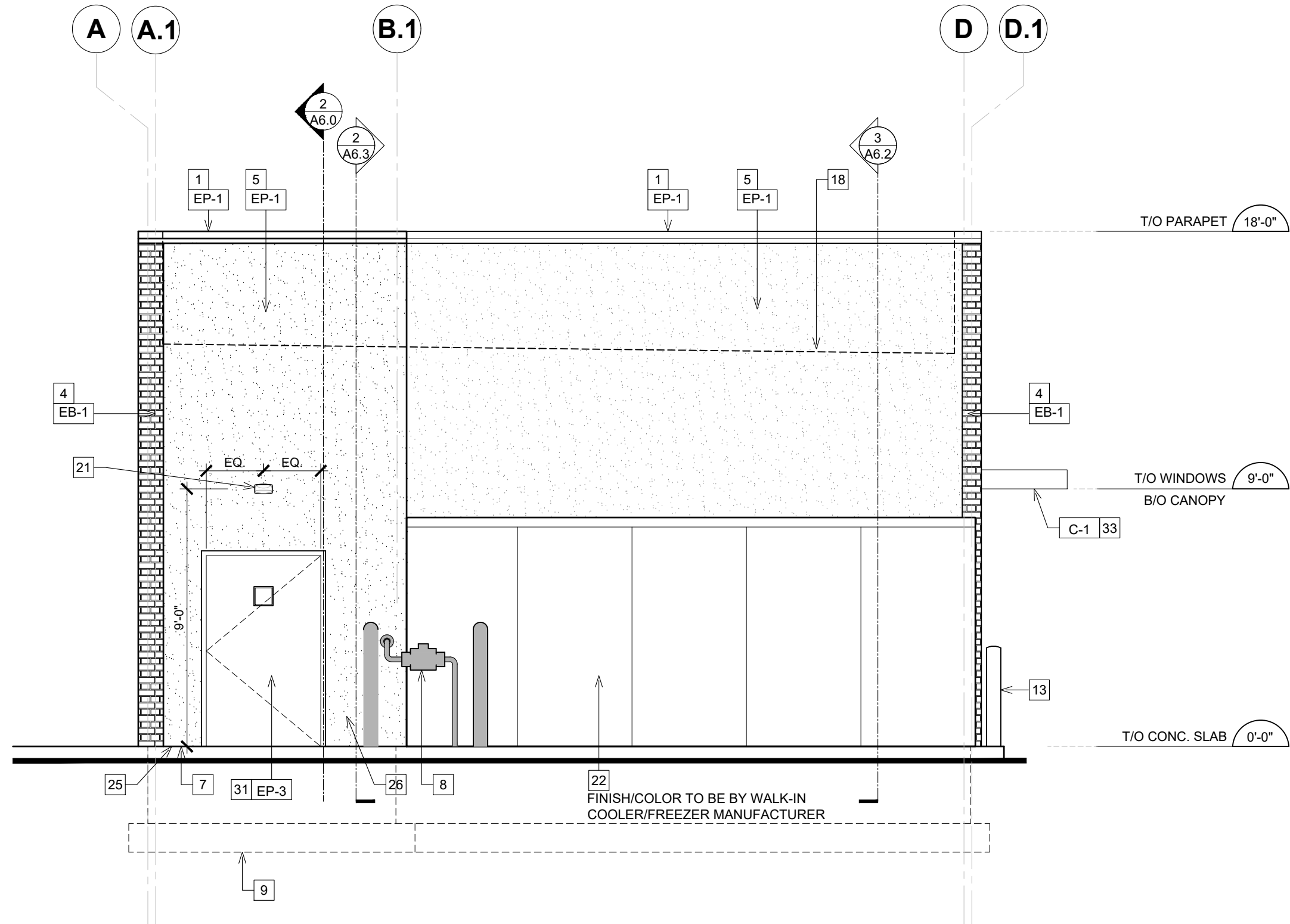
1 A5.1 PROPOSED REAR ELEVATION SCALE: 1/4"=1'-0"
