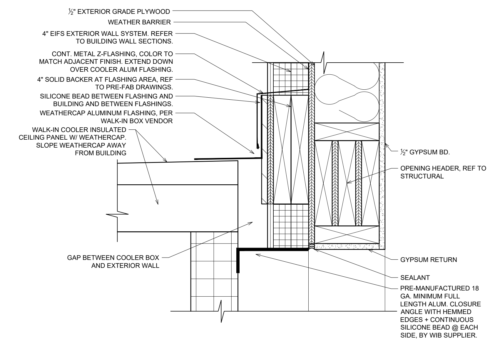
6 HEAD DETAIL @ W.I.B. A8 SCALE: 2 1/2"=1'-0"
