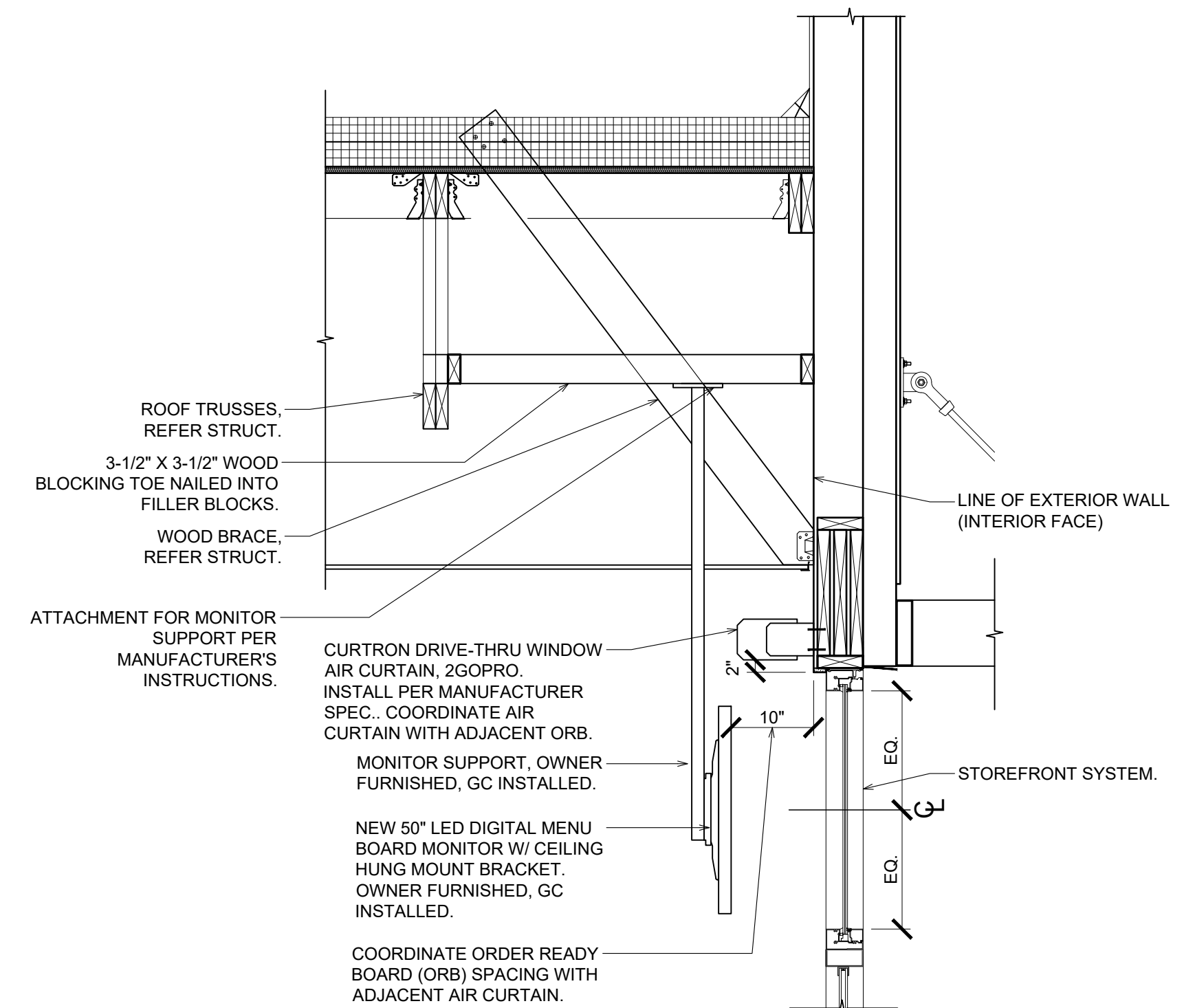
5 MONITOR SUPPORT BRACKET DETAIL A8 SCALE: 3/4" = 1'-0"
