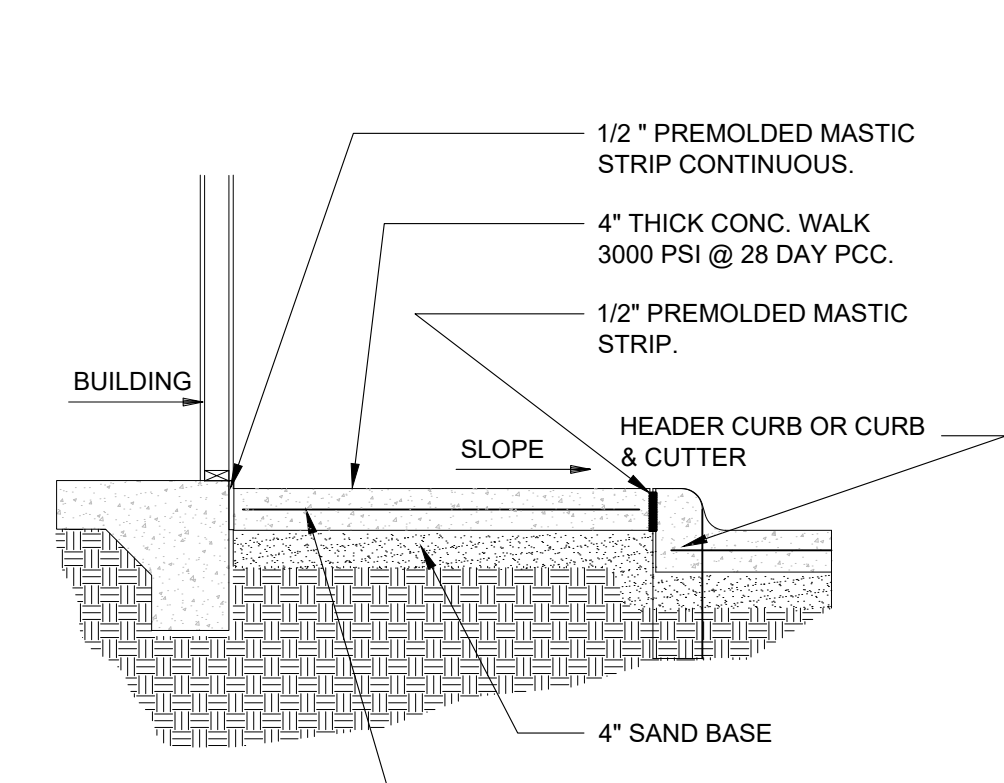
9 SIDEWALK DETAIL AS2.3 SCALE: 3/8" = 1'-0"
