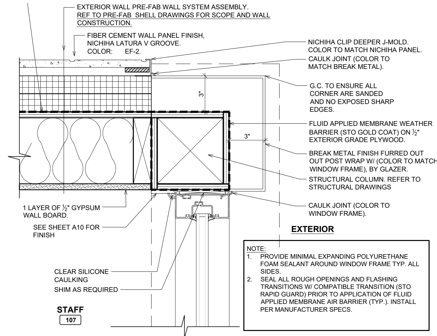
1 PLAN DETAIL @ CORNER A7.2 SCALE: 2 1/2"=1'-0"
