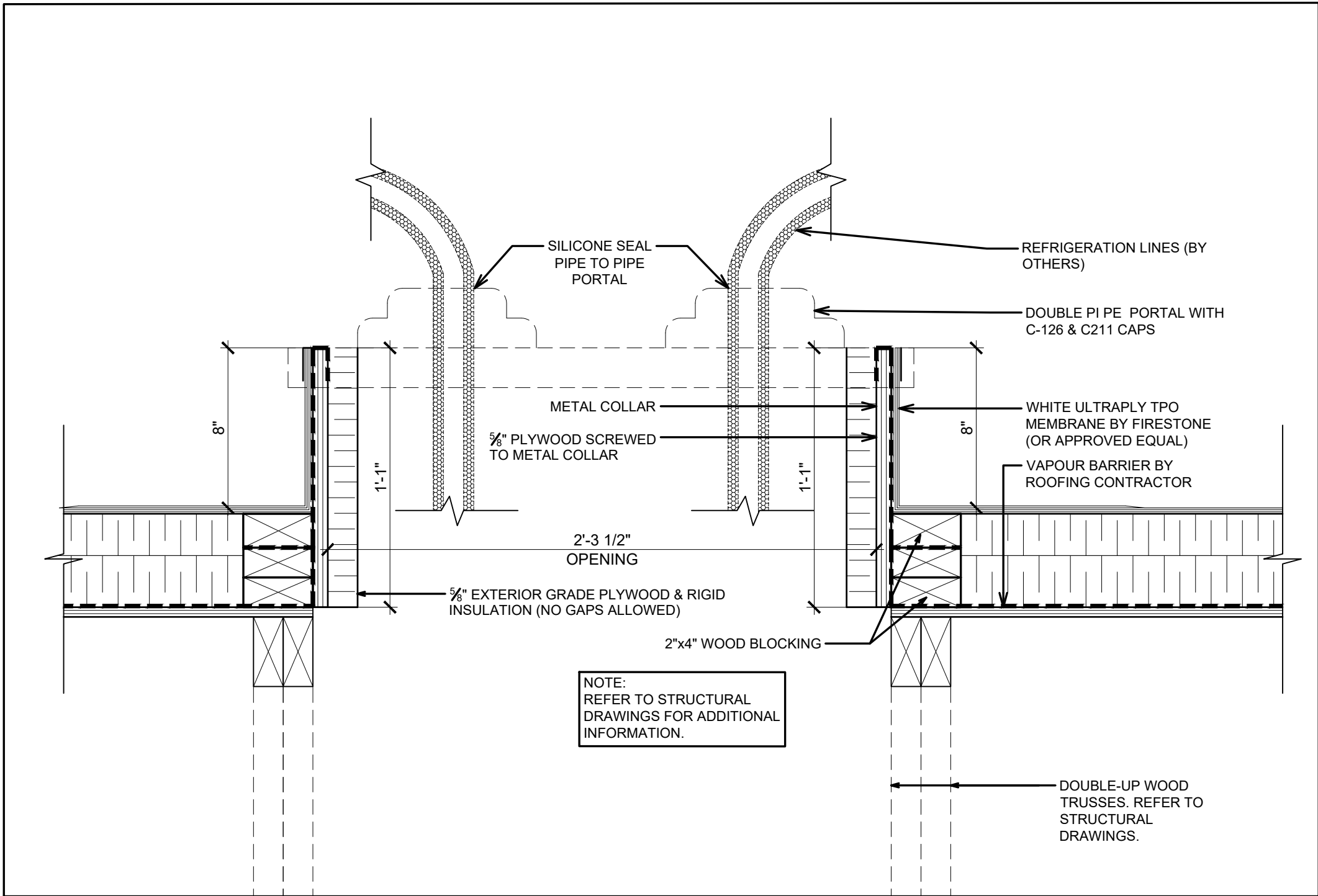
1 A4.1 TYPICAL ROOF OPENING DETAIL AT PIPE PORTAL SCALE: 2"=1'-0"
