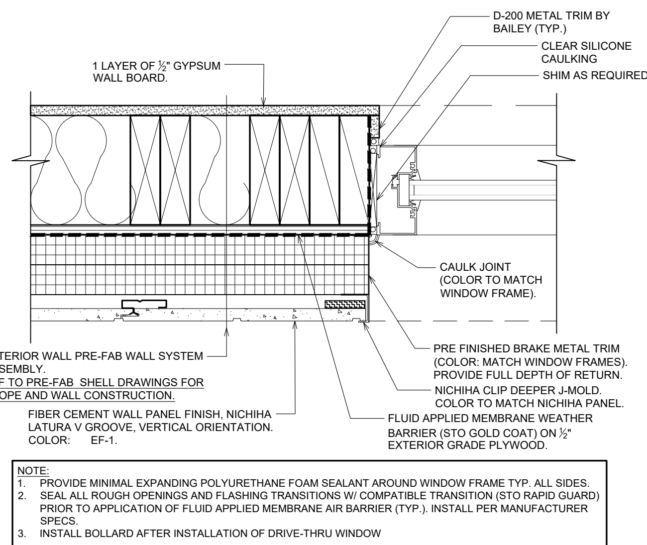
3 PLAN DETAIL @ DRIVE-THRU WINDOW A7.2 SCALE: 2 1/2"=1'-0"
