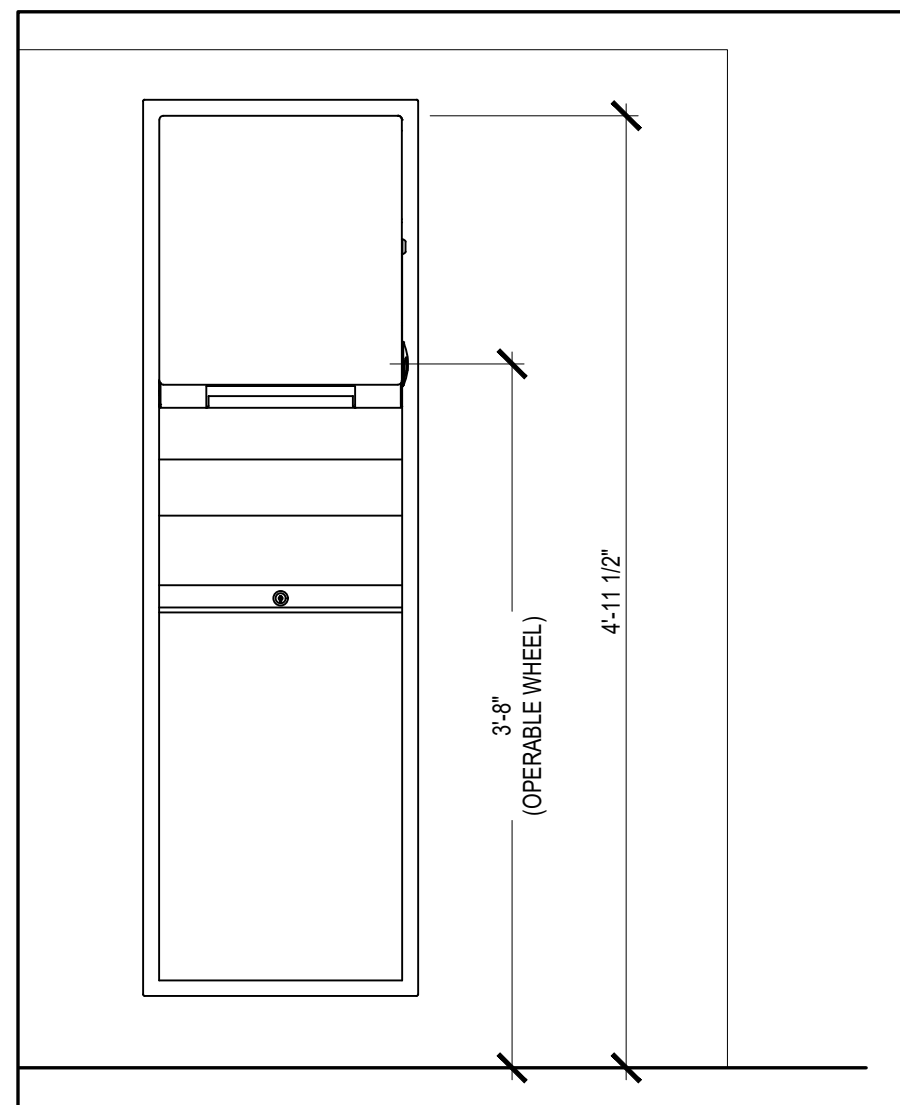
8 DETAIL @ SEMI-RECESSED A9.3 GARBAGE SCALE: 1" = 1'-0"
