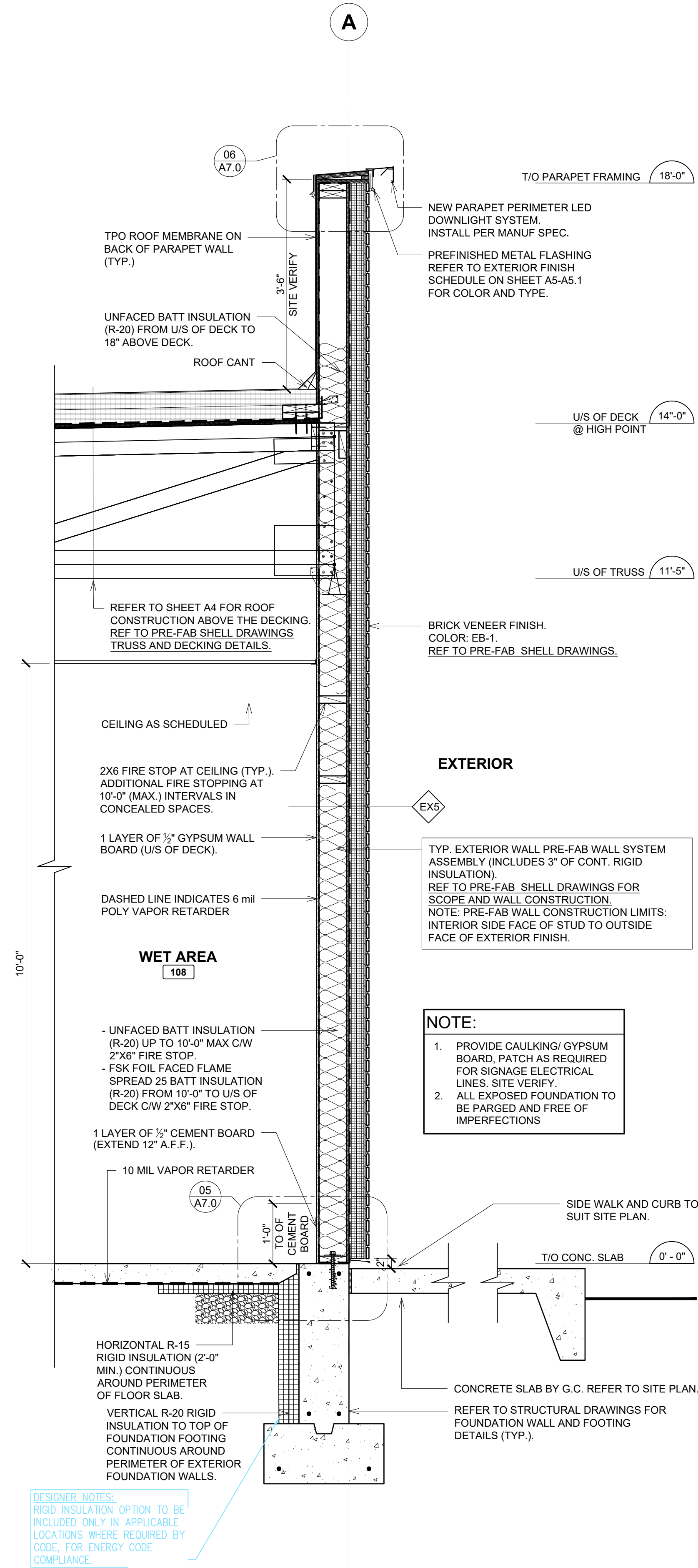
3 WALL SECTION @ SIDE SCALE: 3/4" = 1'-0"
