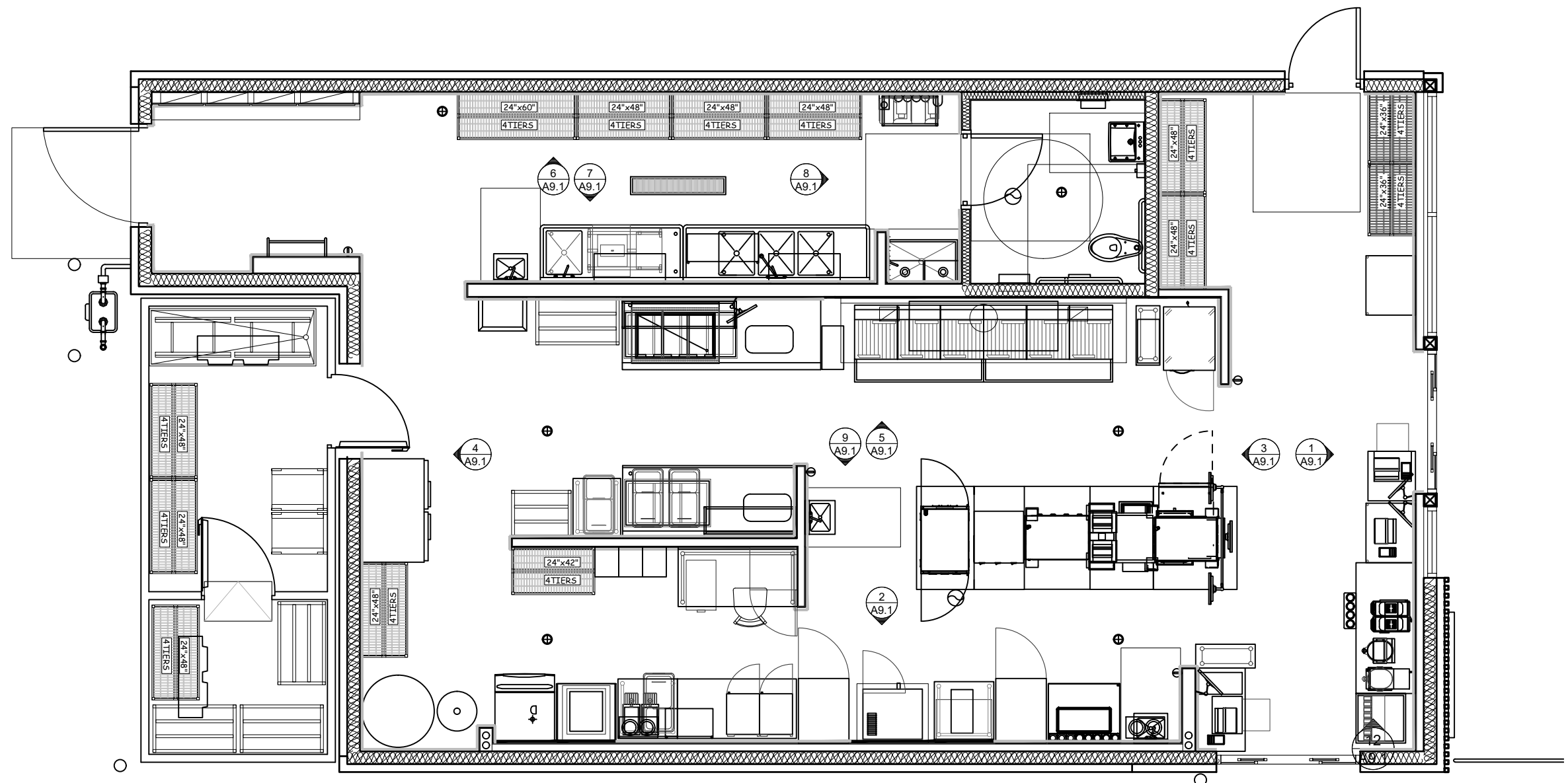
10 LEGEND FLOOR PLAN A9.1 SCALE: 3/16"=1'-0"
