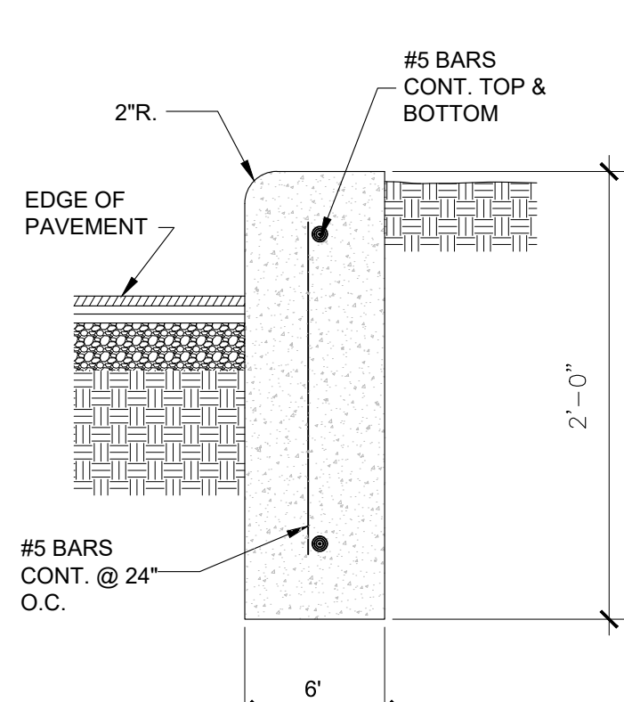
11 CURB DETAIL AS2.3 SCALE: 3/8" = 1'-0"
