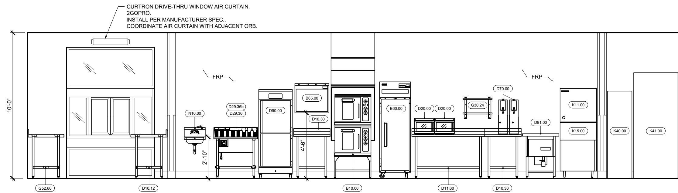
2 SERVICE / PREP AREA A9.1 SCALE: 1/4" = 1'-0"
