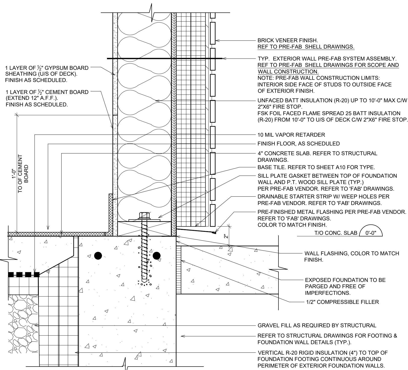
05 SECTION DETAIL @ WALL BASE A7.0 SCALE: 2-1/2" = 1' - 0"
