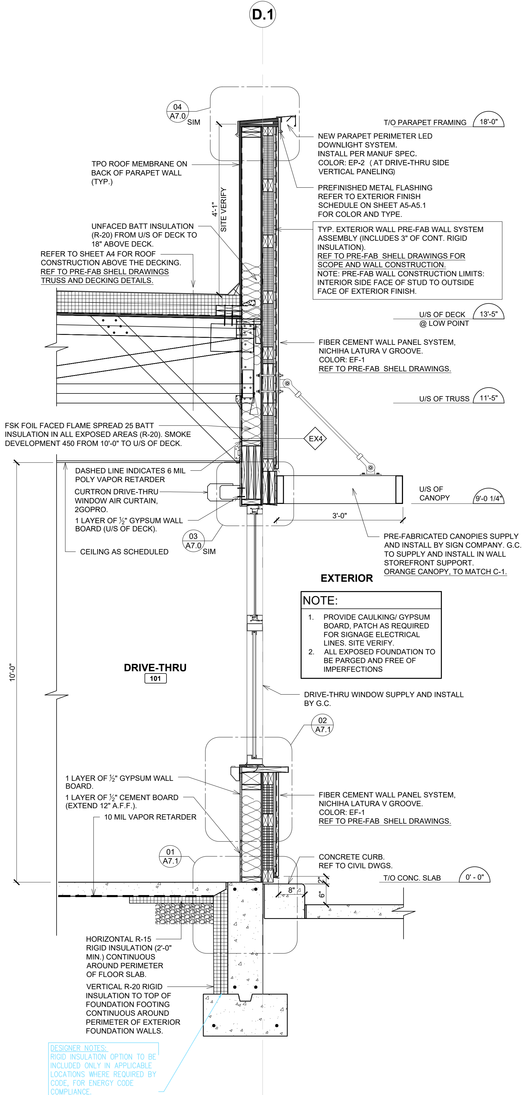
2 WALL SECTION @ DT WINDOW SCALE: 3/4" = 1'-0"
