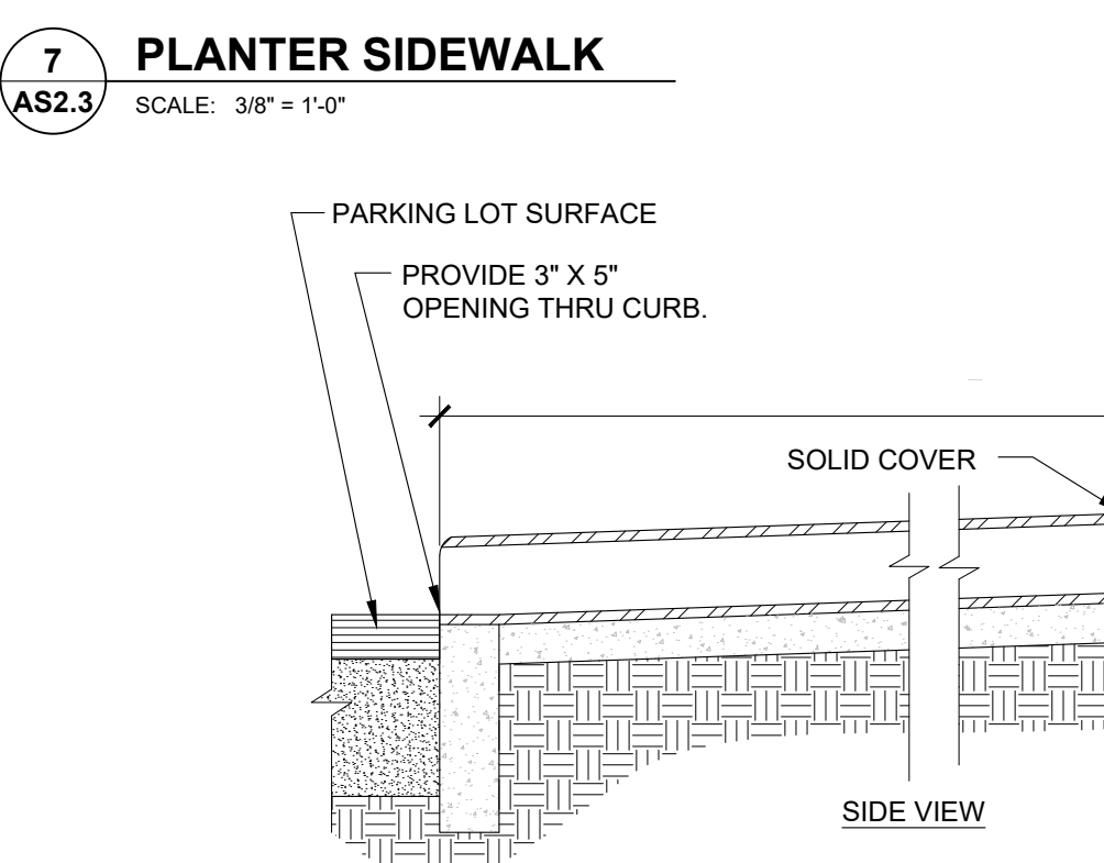
7 PLANTER SIDEWALK AS2.3 SCALE: 3/8" = 1'-0"
