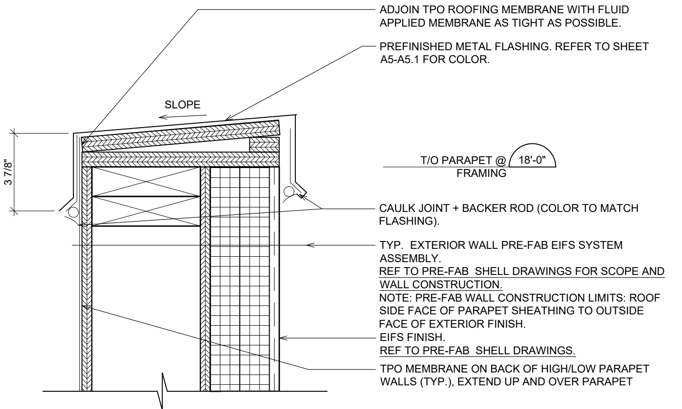
08 SECTION DETAIL @ PARAPET A7.0 SCALE: 2-1/2" = 1' - 0"
