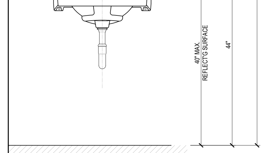
14 MIRROR AND SOAP DISPENSER DETAIL A9.3 SCALE: 1" = 1'-0"
