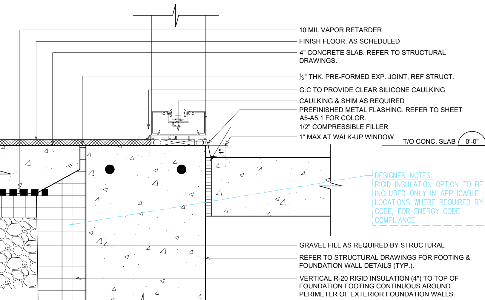
02 SECTION DETAIL @ WALK-UP WINDOW A7.0 SCALE: 2-1/2" = 1' - 0"
