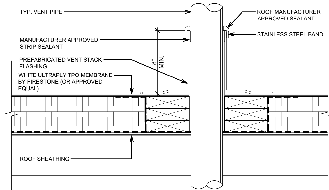
4 VENT PENETRATION DETAIL SCALE: 2"=1'-0"
