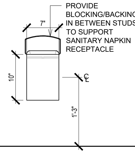
13 DETAIL @ SANITARY NAPKIN A9.3 SCALE: 1" = 1'-0" RECEPTACLE
