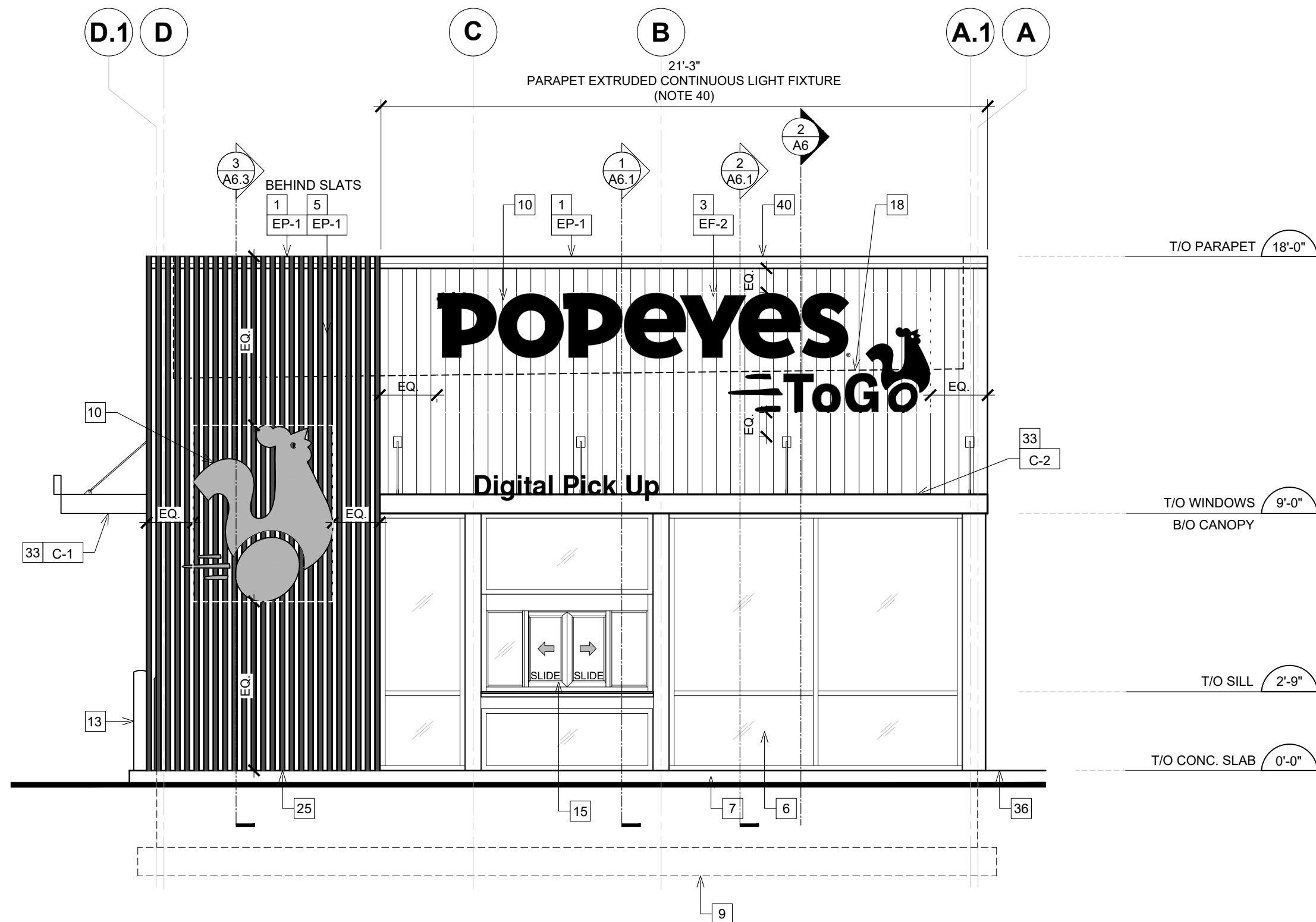
1 PROPOSED FRONT ELEVATION A5 SCALE: 1/4"=1'-0"
