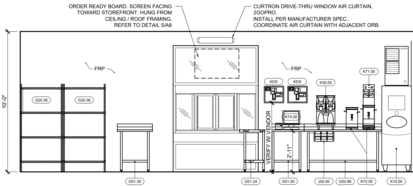
1 SERVICE AREA A9.1 SCALE: 1/4" = 1'-0"
