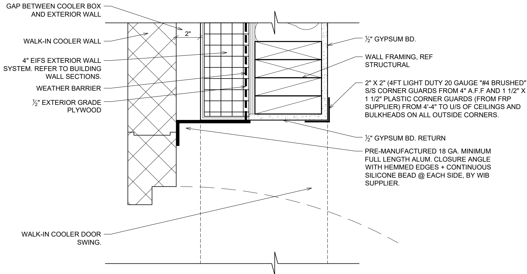
5 FLASHING DETAIL @ W.I.B. DOOR A7.2 SCALE: 2 1/2"=1'-0"
