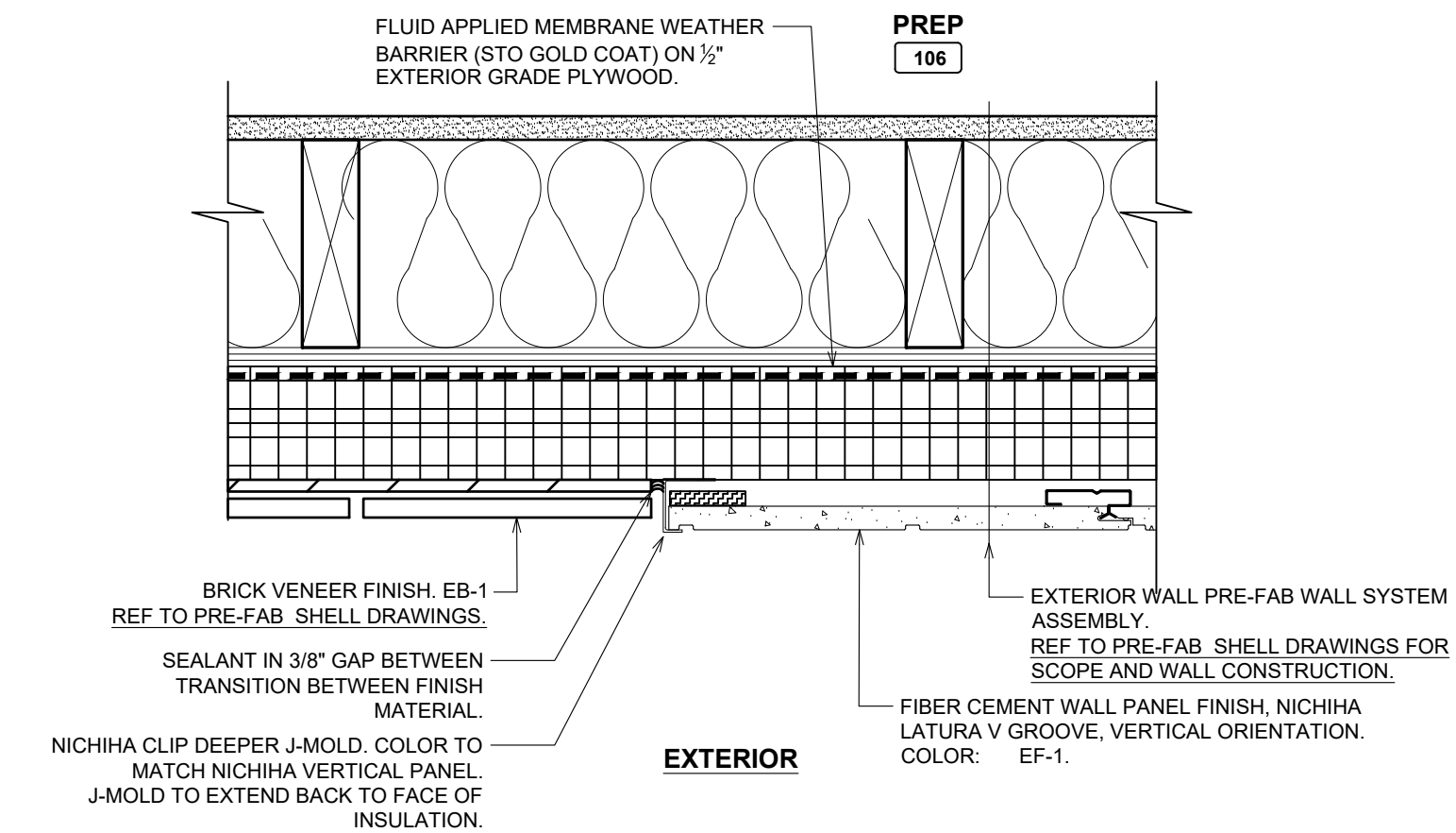
4 PLAN DETAIL @ MATERIAL TRANSITION A7.2 SCALE: 2 1/2"=1'-0"
