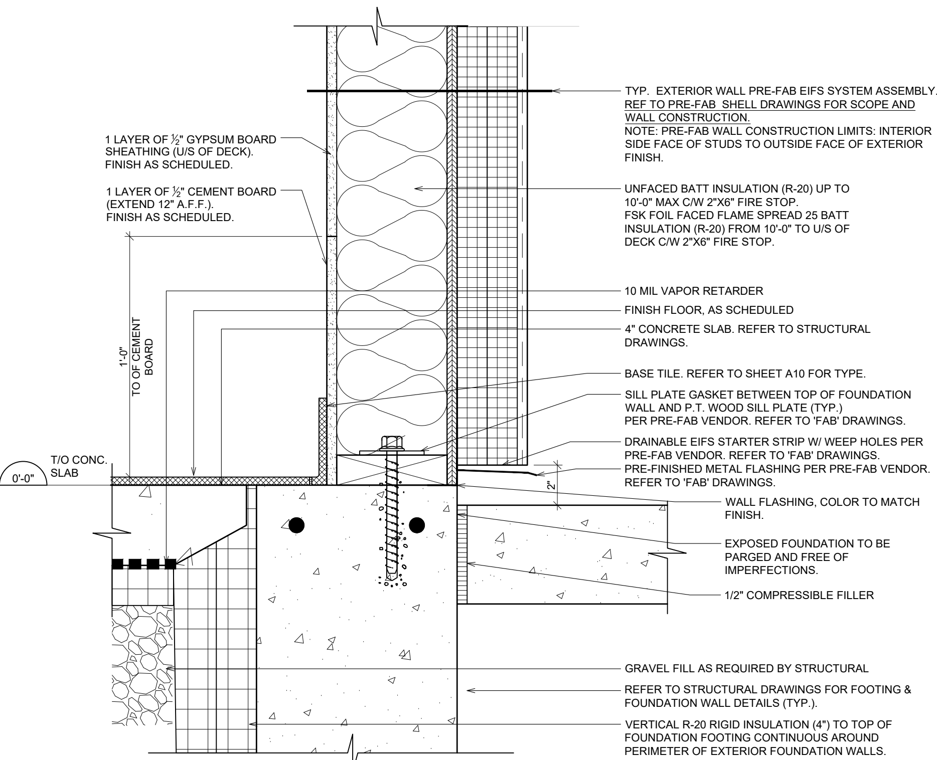
07 SECTION DETAIL @ WALL BASE A7.0 SCALE: 2-1/2" = 1' - 0"
