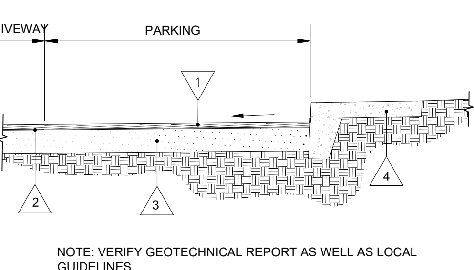
8 TYP. ASPHALT PAVEMENT DETAIL AS2.3 SCALE: 3/8" = 1'-0"
