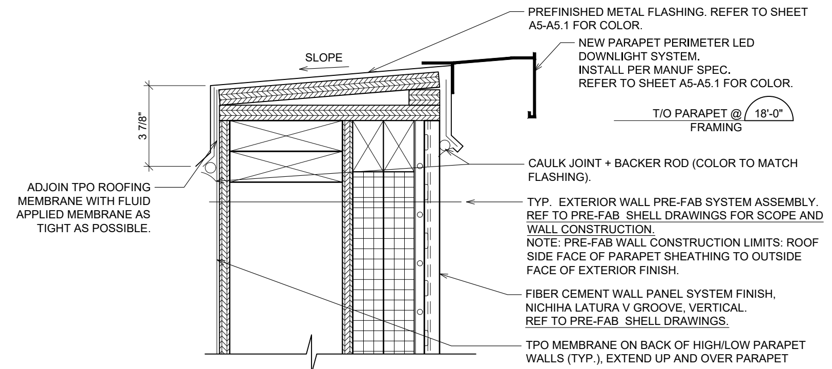
04 SECTION DETAIL @ PARAPET A7.0 SCALE: 2-1/2" = 1' - 0"
