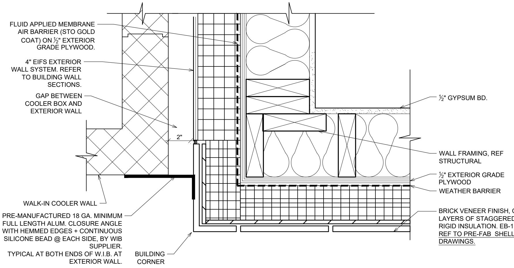
7 FLASHING DETAIL @ W.I.B. CORNER A7.2 SCALE: 2 1/2"=1'-0"
