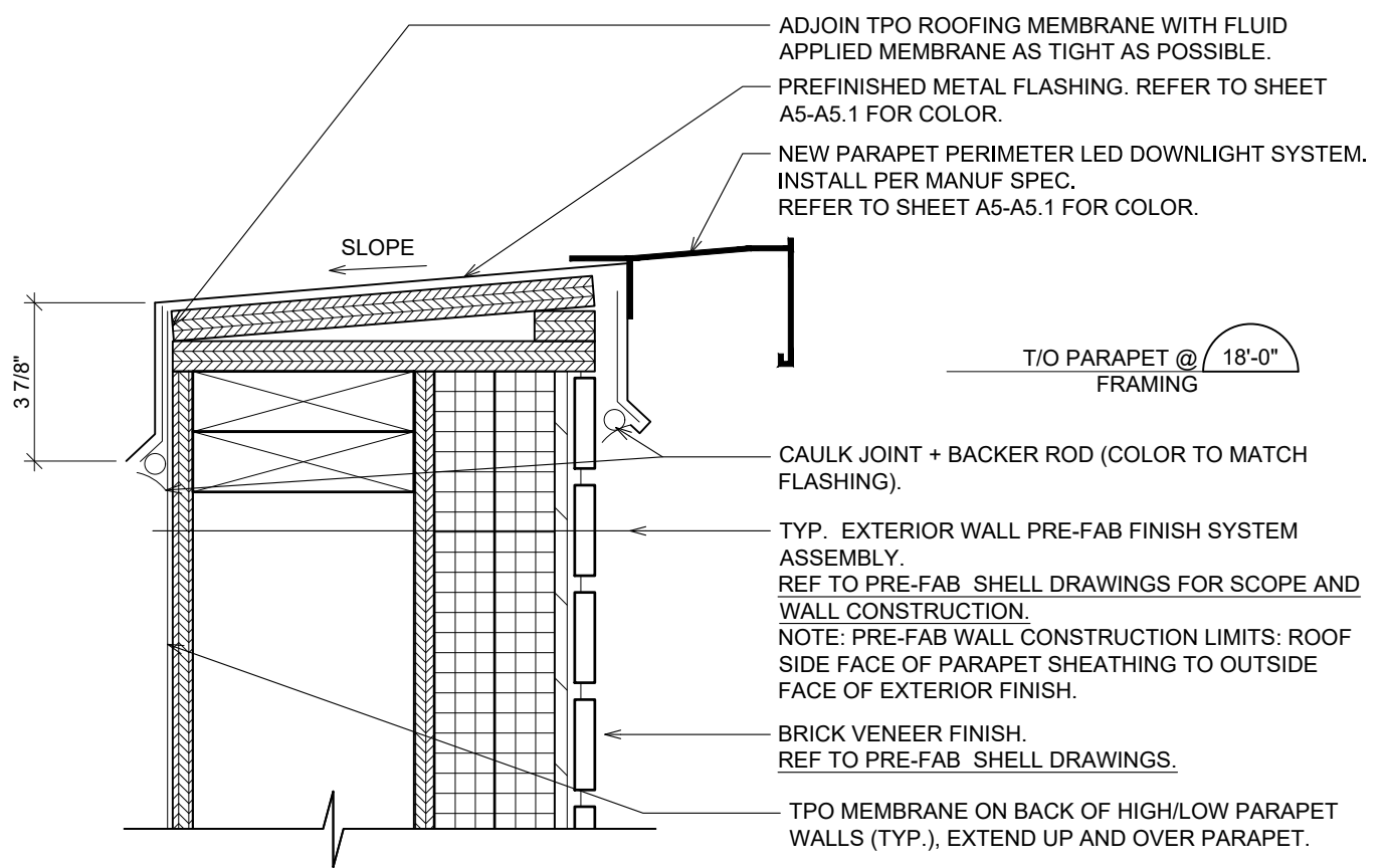
06 SECTION DETAIL @ PARAPET A7.0 SCALE: 2-1/2" = 1' - 0"
