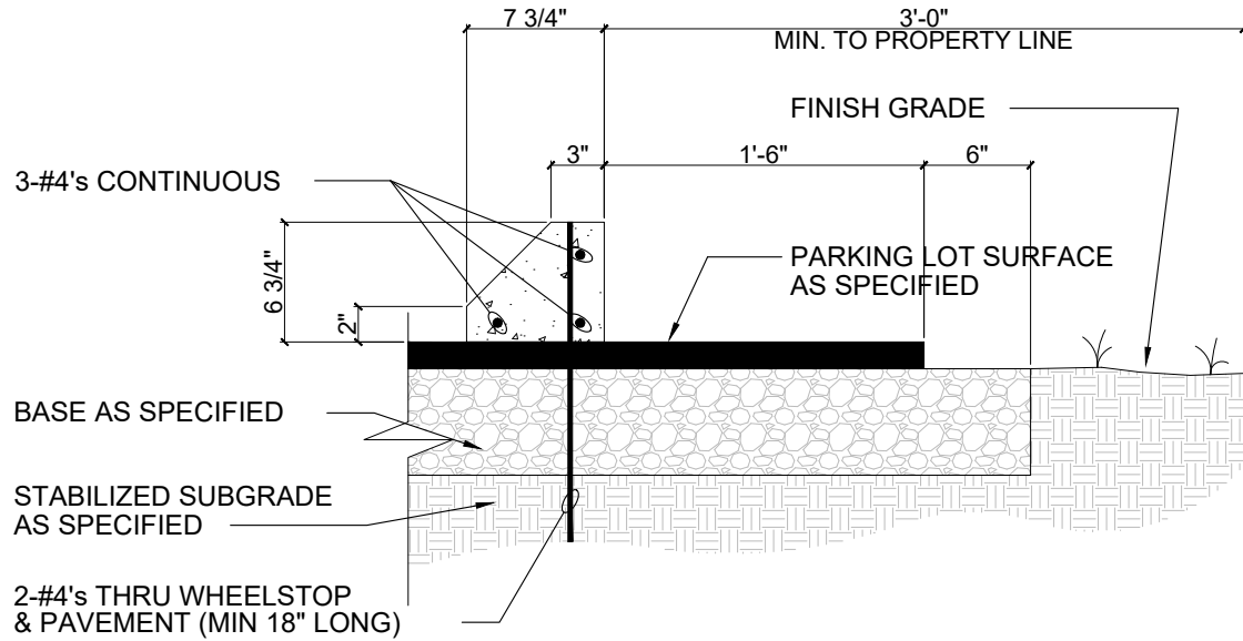
7 WHEELSTOP (PRECAST) SCALE: 1" = 1'-0"
