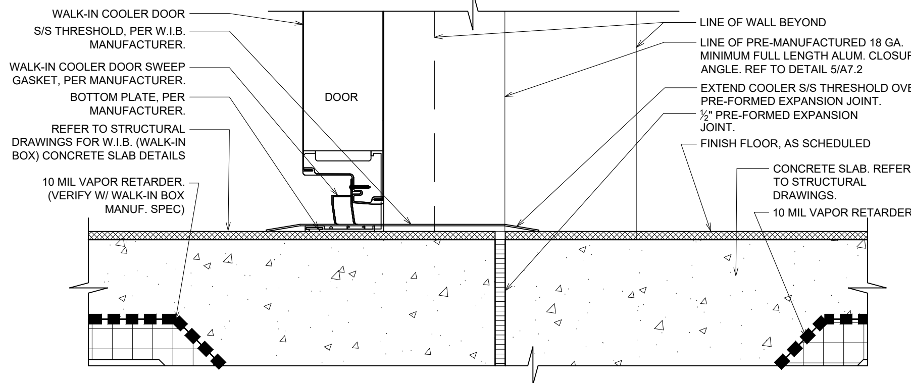
8 THRESHOLD DETAIL @ W.I.B. A7.2 SCALE: 2 1/2"=1'-0"
