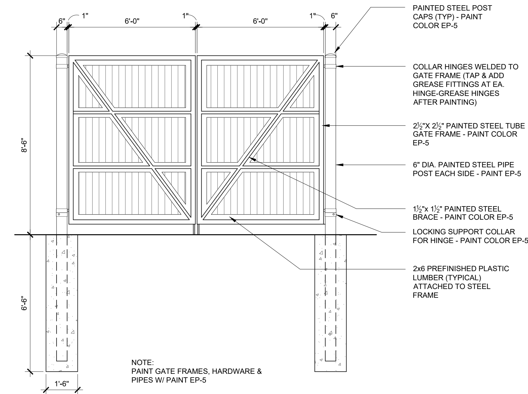
3 DUMPSTER ENCLOSURE & GATE INT. ELEV. SCALE: 3/8" = 1'-0"
