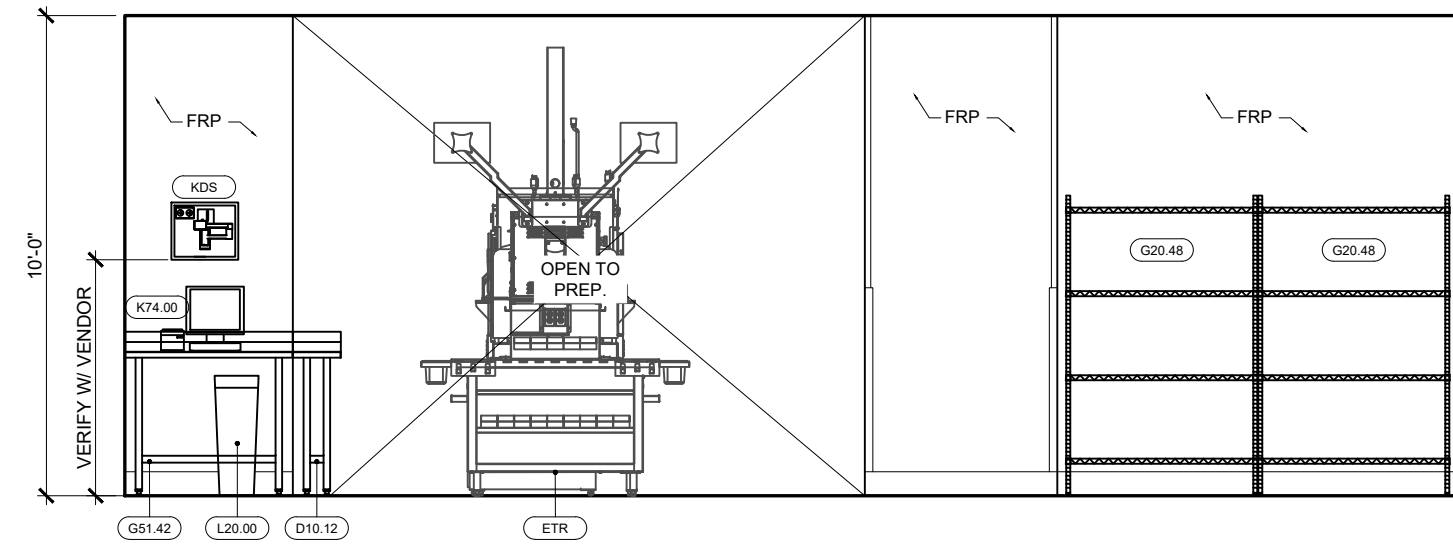
3 PREP / STAFF AREA A9.1 SCALE: 1/4" = 1'-0"
