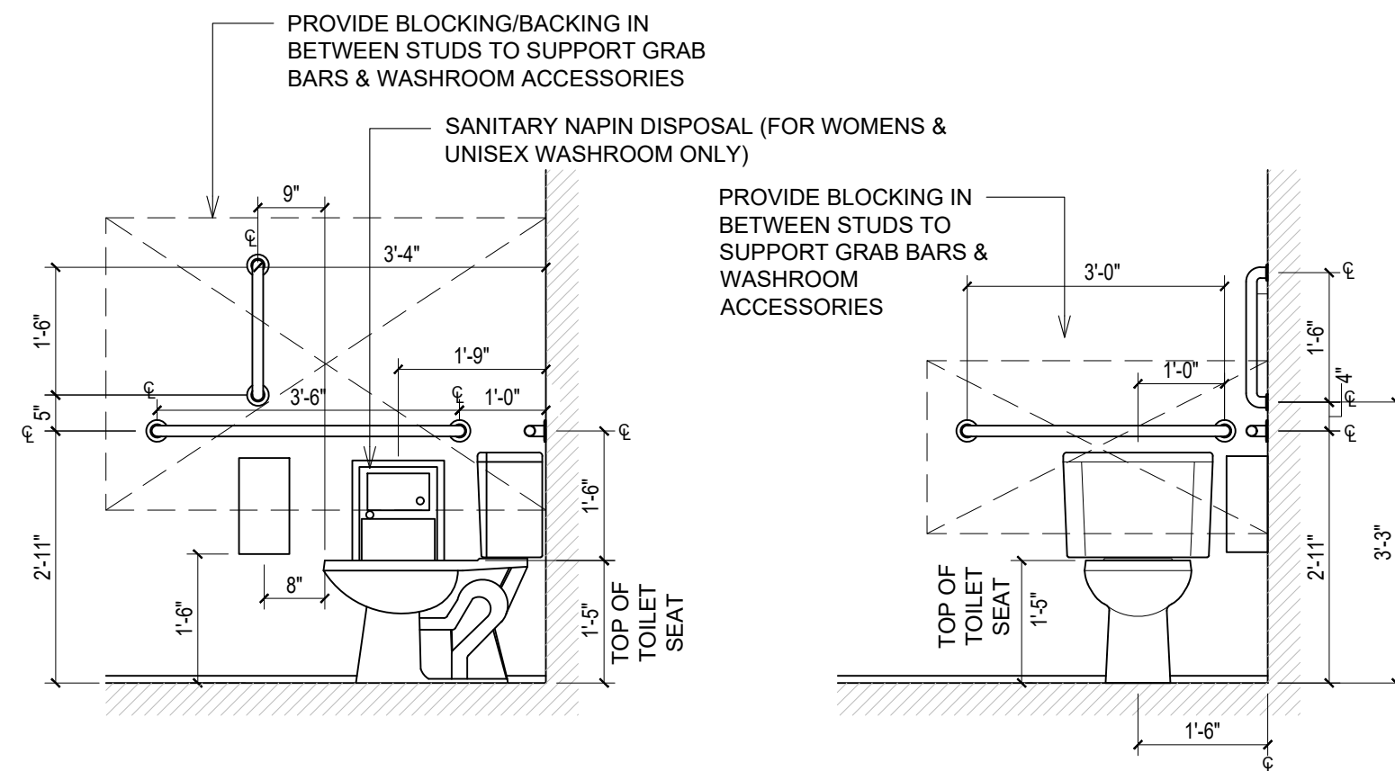
11 A9.3 DETAIL @ GRAB BARS SCALE: 1/2" = 1'-0"
