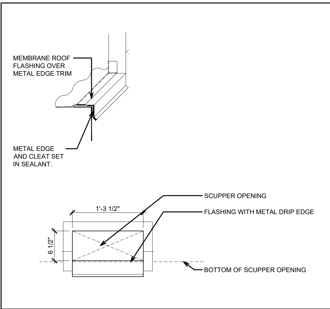
2 A4.1 EMERGENCY OVERFLOW SCUPPER DETAIL SCALE: 1"=1'-0"
