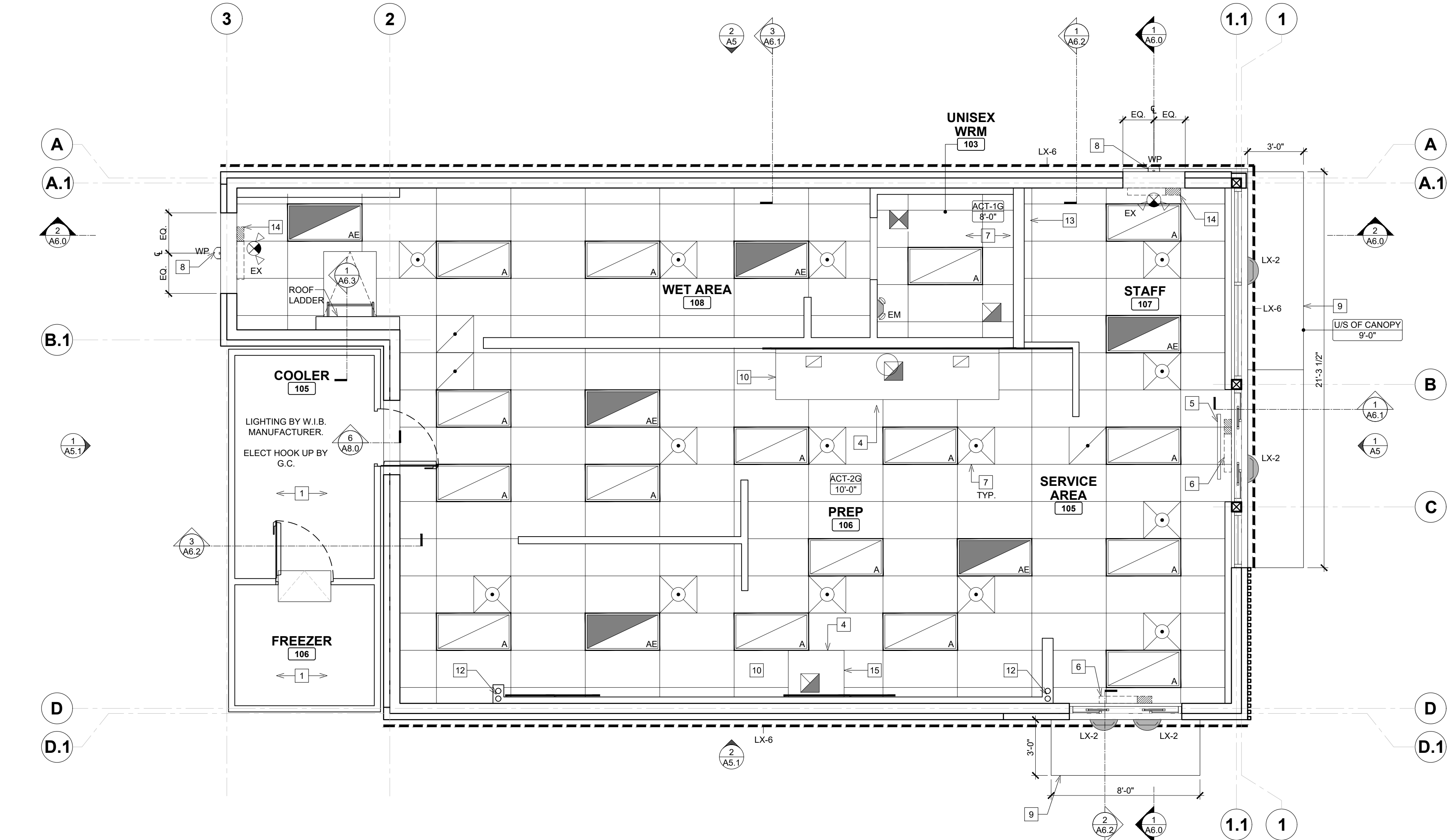
1 A3 REELECTED CEILING PLAN SCALE: 1/4"=1'-0"
