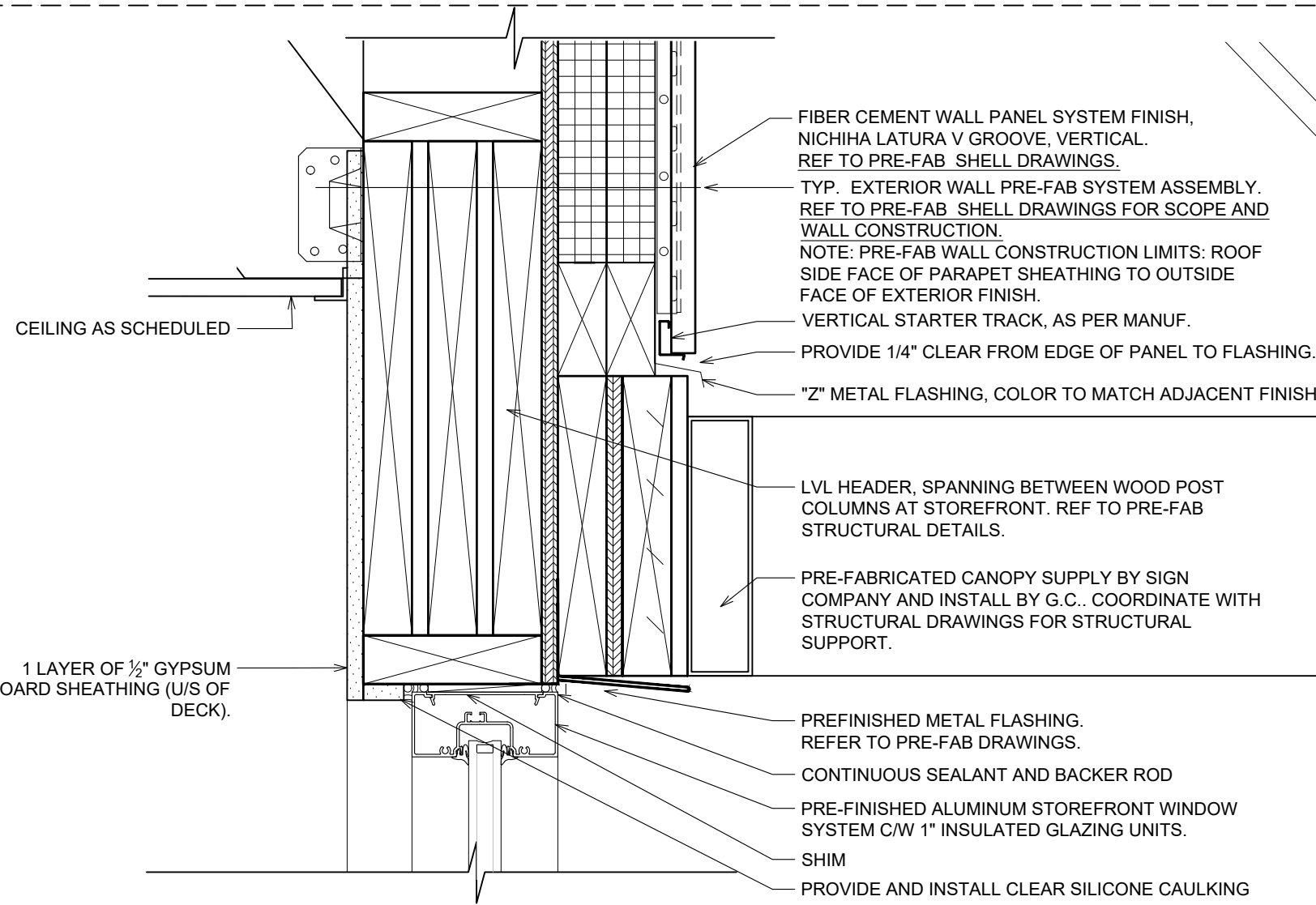
03 SECTION DETAIL @ STOREFRONT HEAD A7.0 SCALE: 2-1/2" = 1' - 0"
