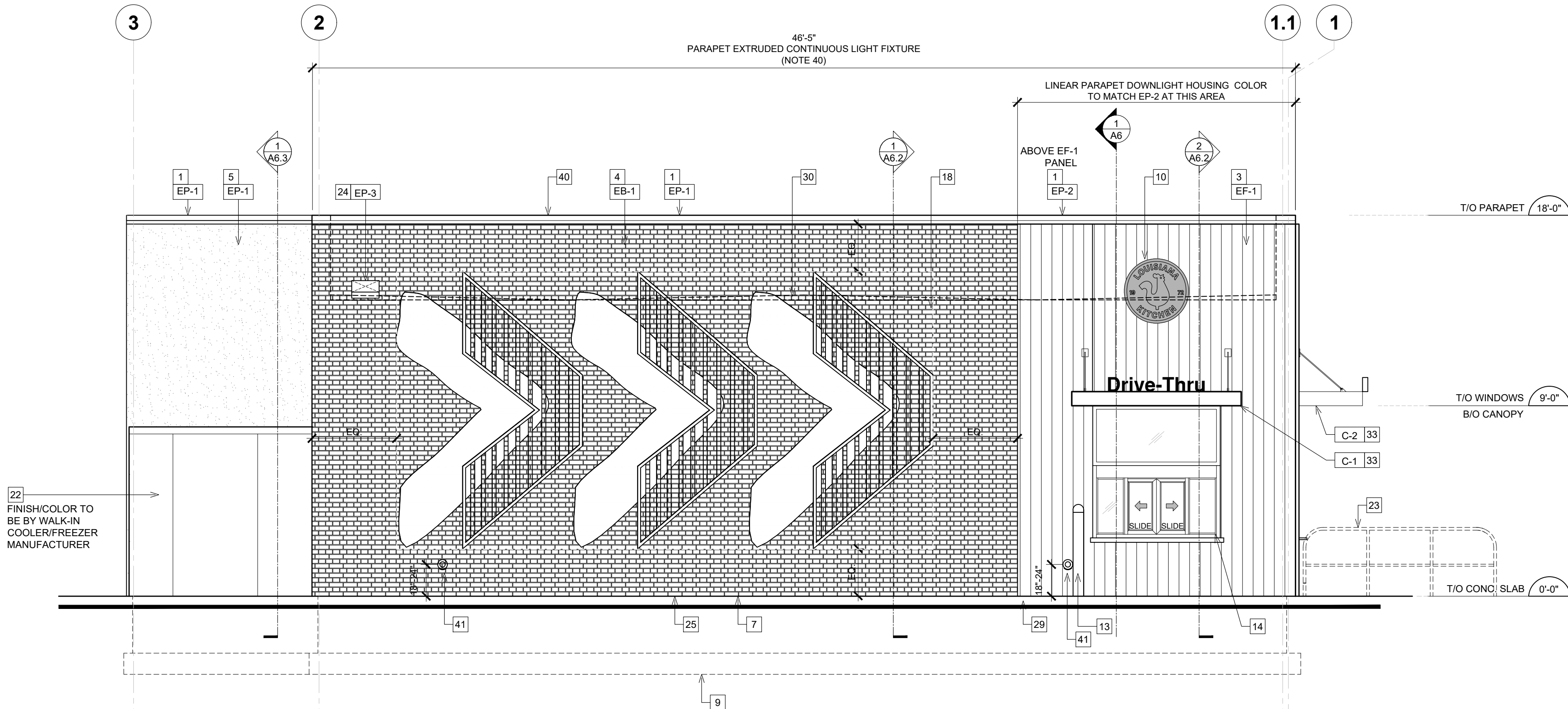
2 A5.1 PROPOSED DT ELEVATION SCALE: 1/4"=1'-0"
