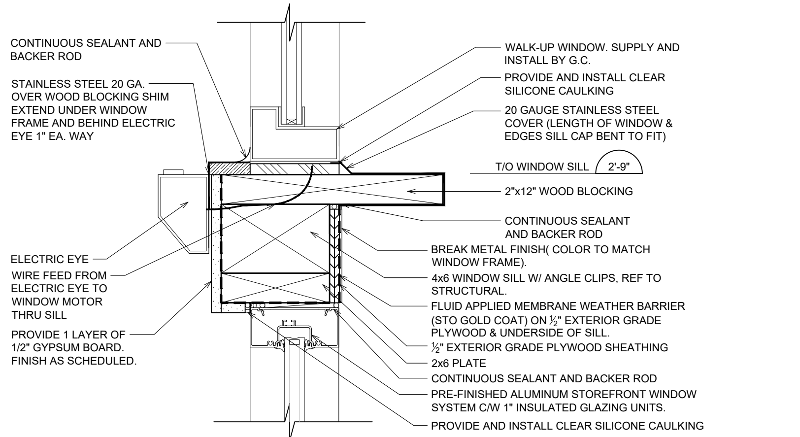
02 SECTION DETAIL @ WALK-UP WINDOW A7.0 SCALE: 2-1/2" = 1' - 0"
