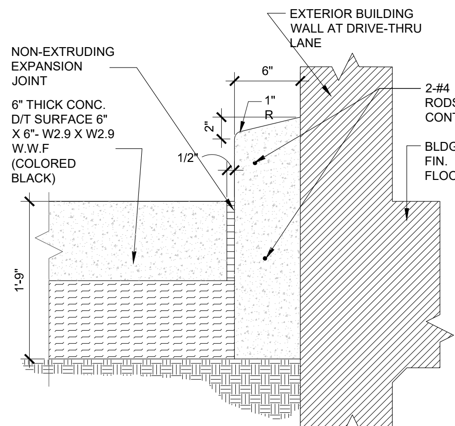
5 6" BARRIER CURB @ DRIVE-THRU WINDOW AS2.3 SCALE: 3/8" = 1'-0"
