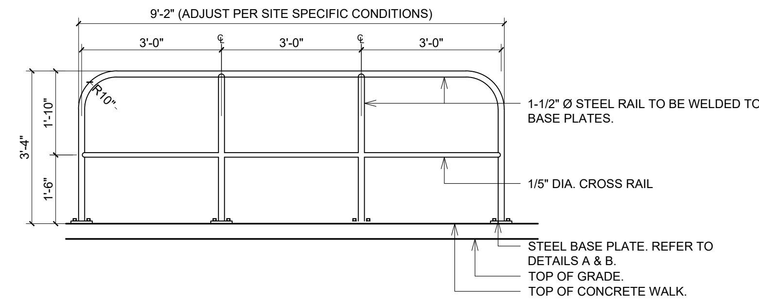
2 DETAIL @ METAL RAILING A8 SCALE: 1/2" = 1'-0"
