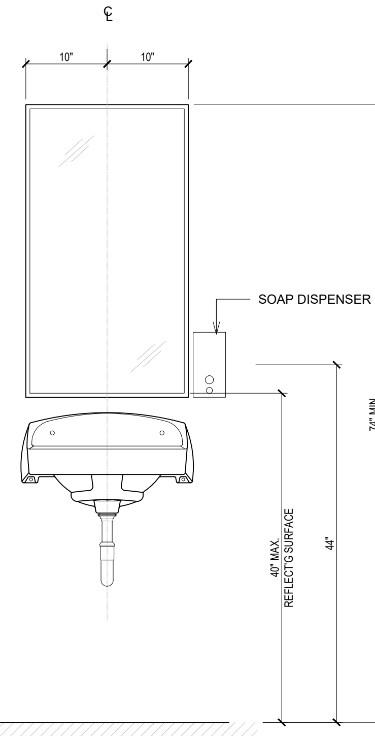
14 MIRROR AND SOAP DISPENSER DETAIL A9.3 SCALE: 1" = 1'-0"
