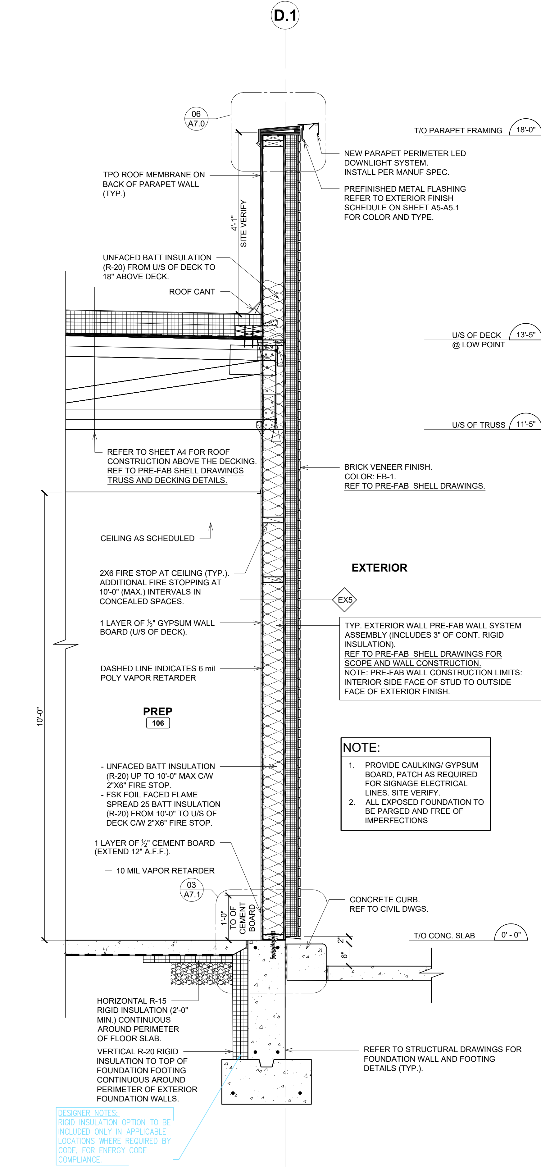
1 WALL SECTION @ DT ELEVATION SCALE: 3/4" = 1'-0"
