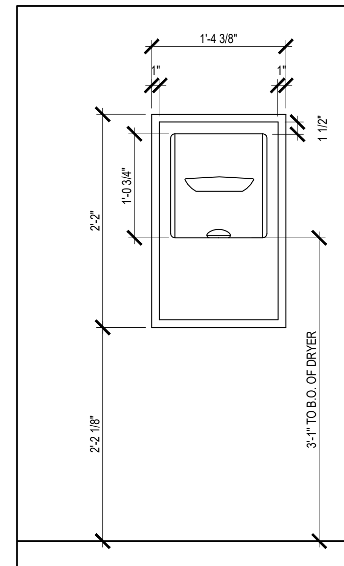
10 DETAIL @ HAND DRYER A9.3 SCALE: 1" = 1'-0"
