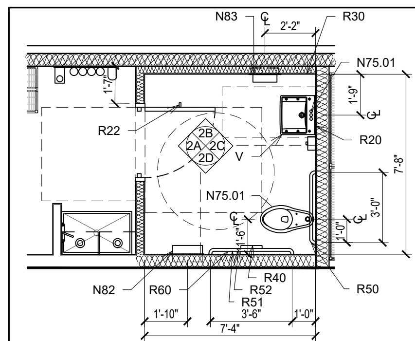
1 PLAN UNISEX WASHROOM A9.3 SCALE: 1/4" = 1'-0"
