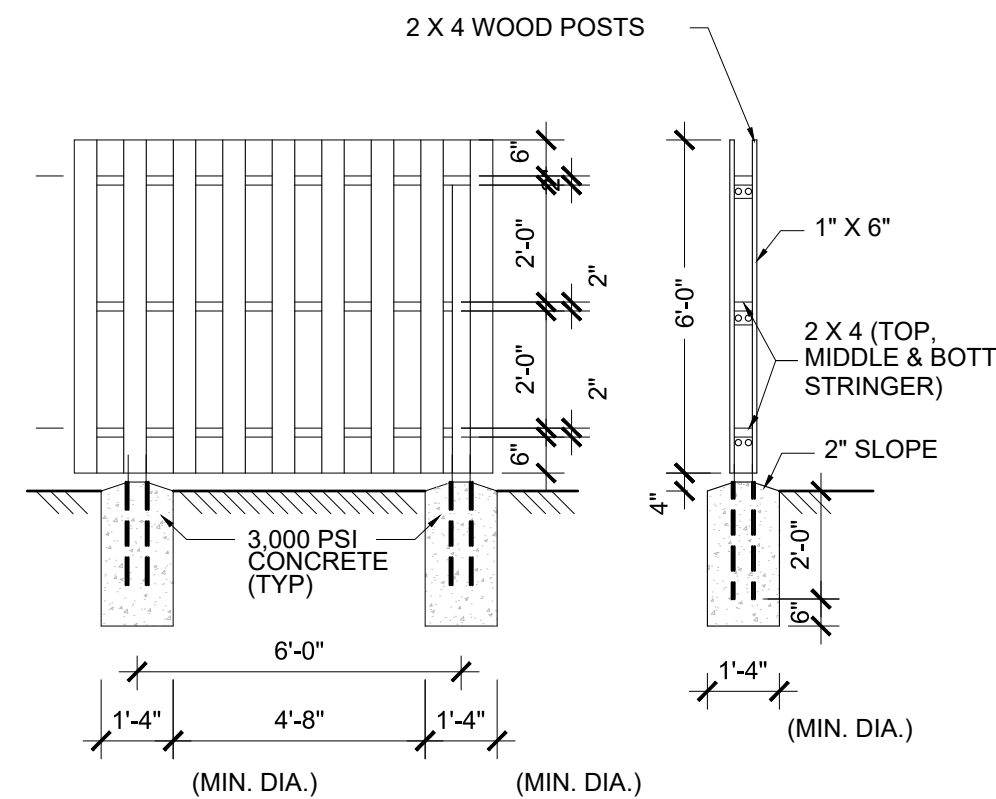
1 SHADOW BOX WOOD FENCE AS2.3 SCALE: 3/8" = 1'-0"
