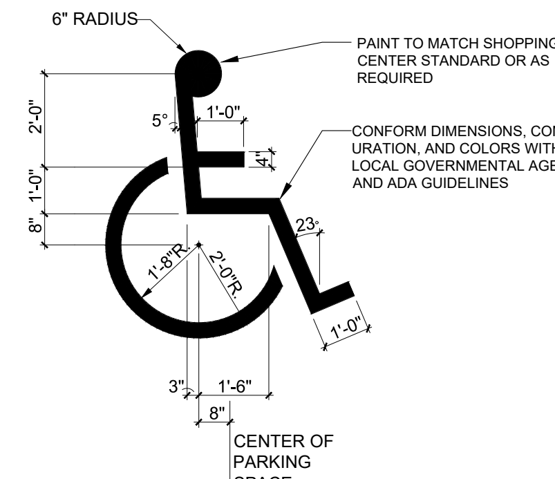
12 HANDICAP SYMBOL AS2.3 SCALE: 3/8" = 1'-0"
