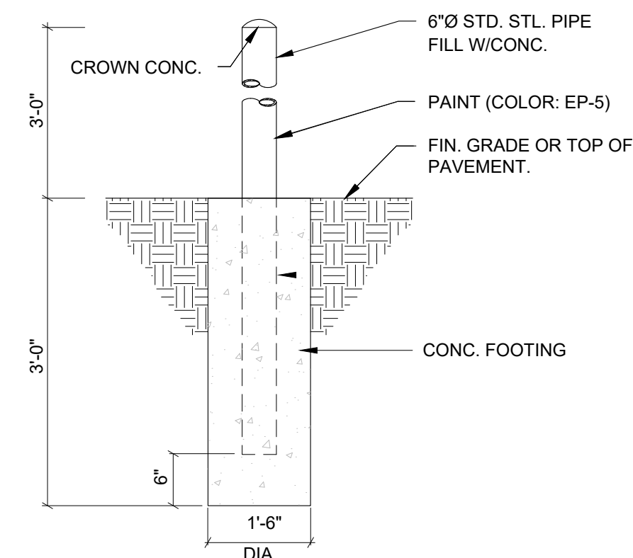
15 BOLLARD DETAIL AS2.3 SCALE: 3/8" = 1'-0"
