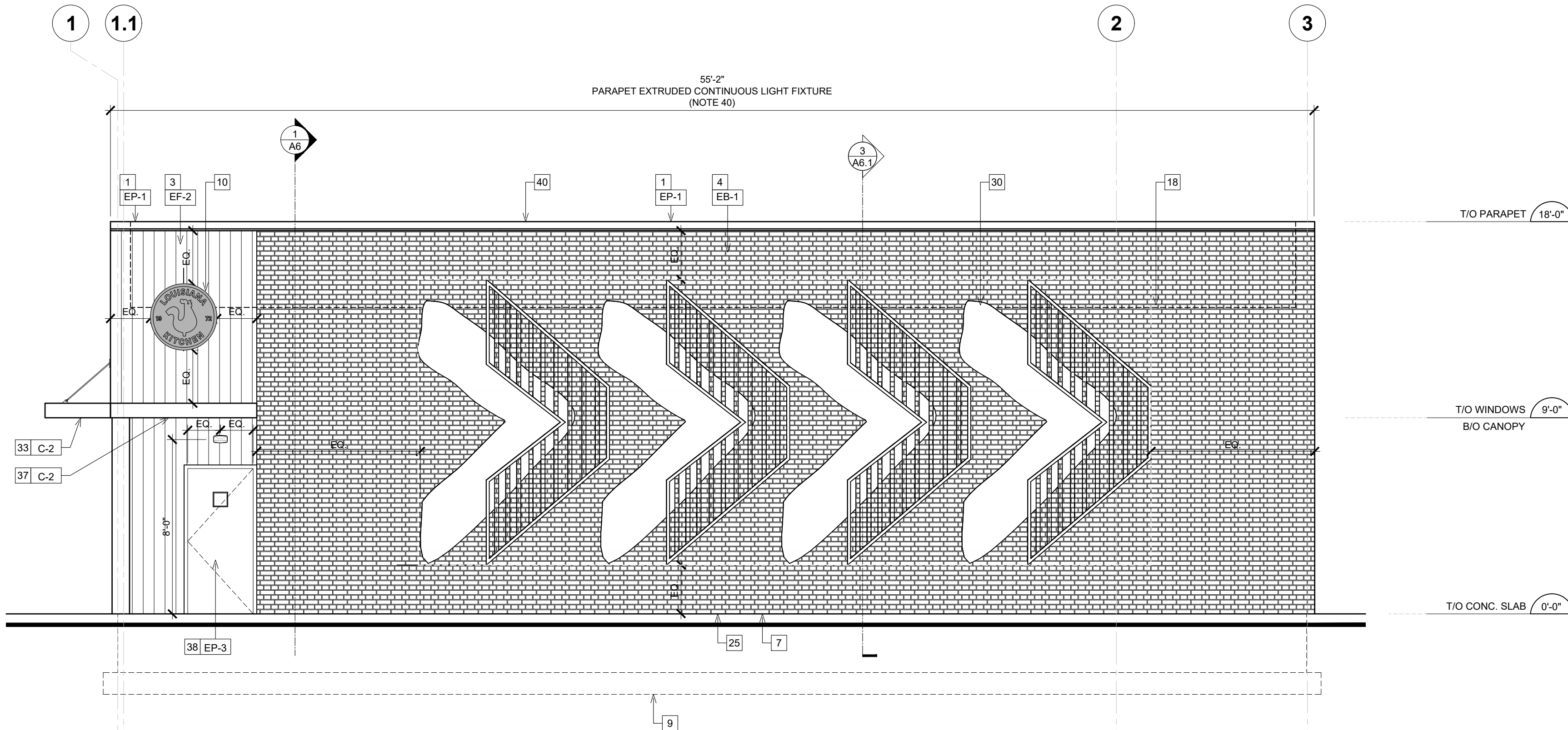
2 PROPOSED SIDE (NON-DT) ELEVATION A5 SCALE: 1/4"=1'-0"
