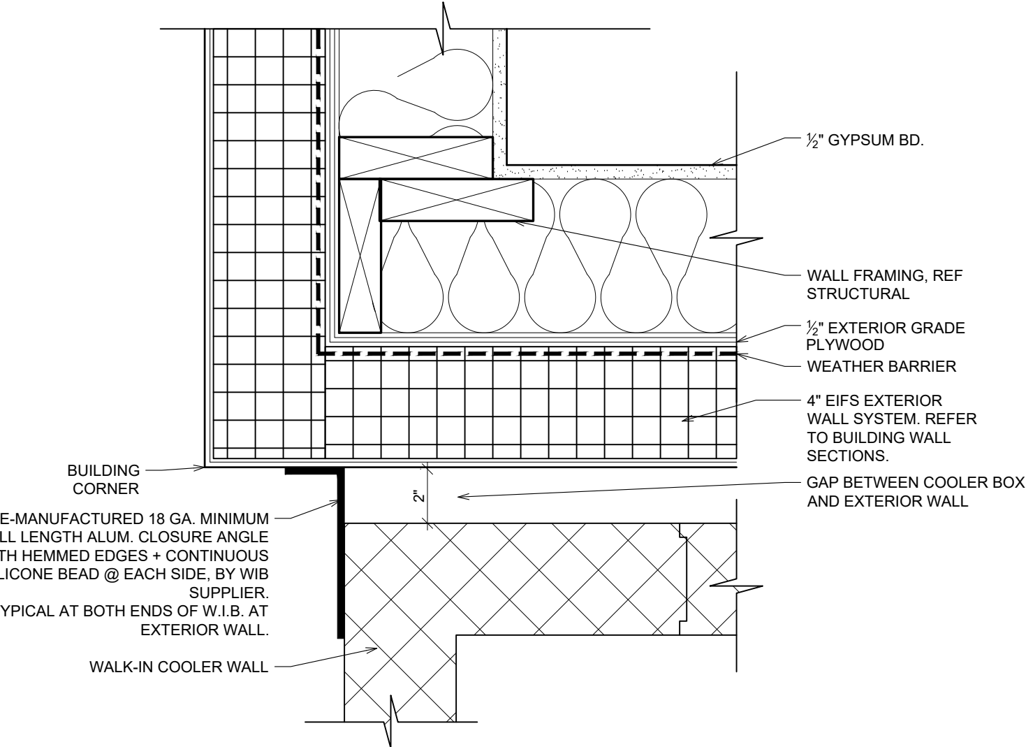
6 FLASHING DETAIL @ W.I.B. CORNER A7.2 SCALE: 2 1/2"=1'-0"
