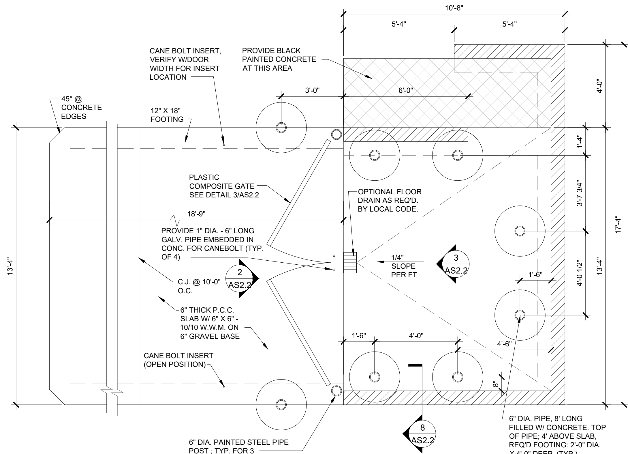
1 STANDARD DUMPSTER ENCLOSURE (SINGLE) SCALE: 3/8" = 1'-0"
