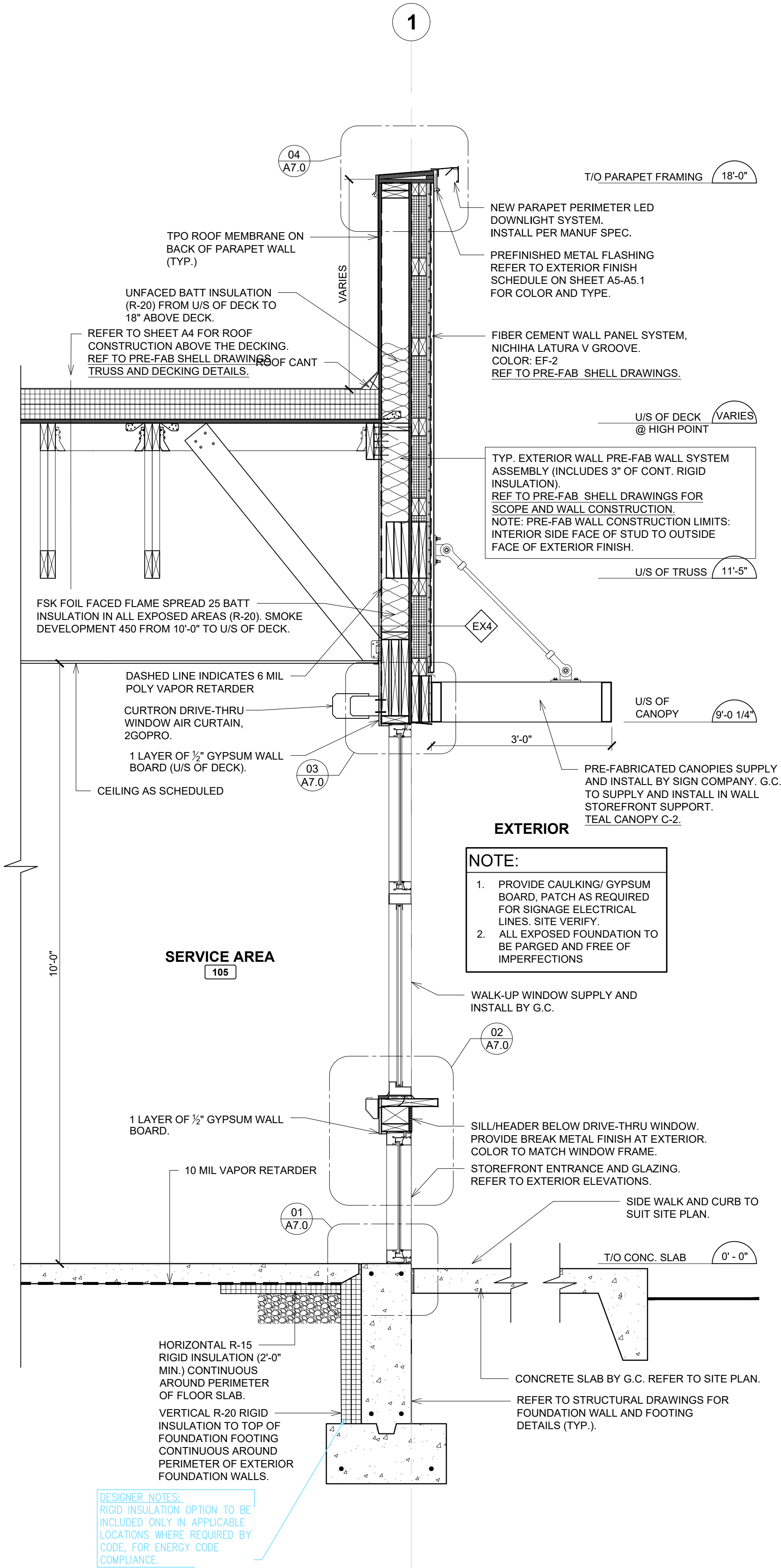
1 WALL SECTION @ WALK-UP WINDOW SCALE: 3/4" = 1'-0"
