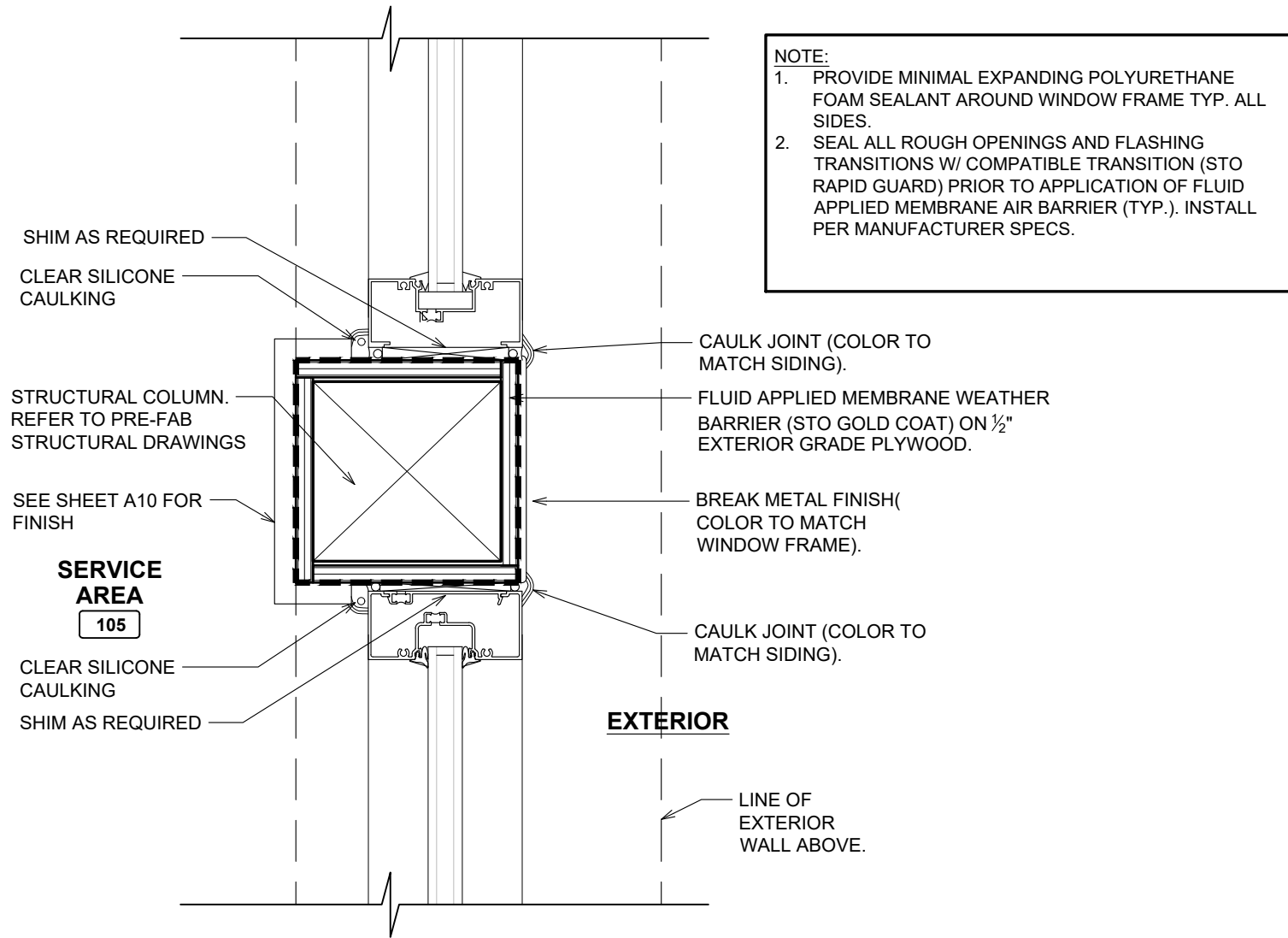
2 PLAN DETAIL @ STOREFRONT POST A7.2 SCALE: 2 1/2"=1'-0"
