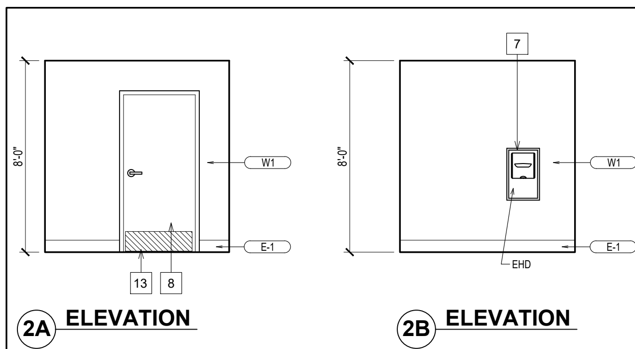
2 ELEVATIONS UNISEX WASHROOM A9.3 SCALE: 1/4" = 1'-0"
