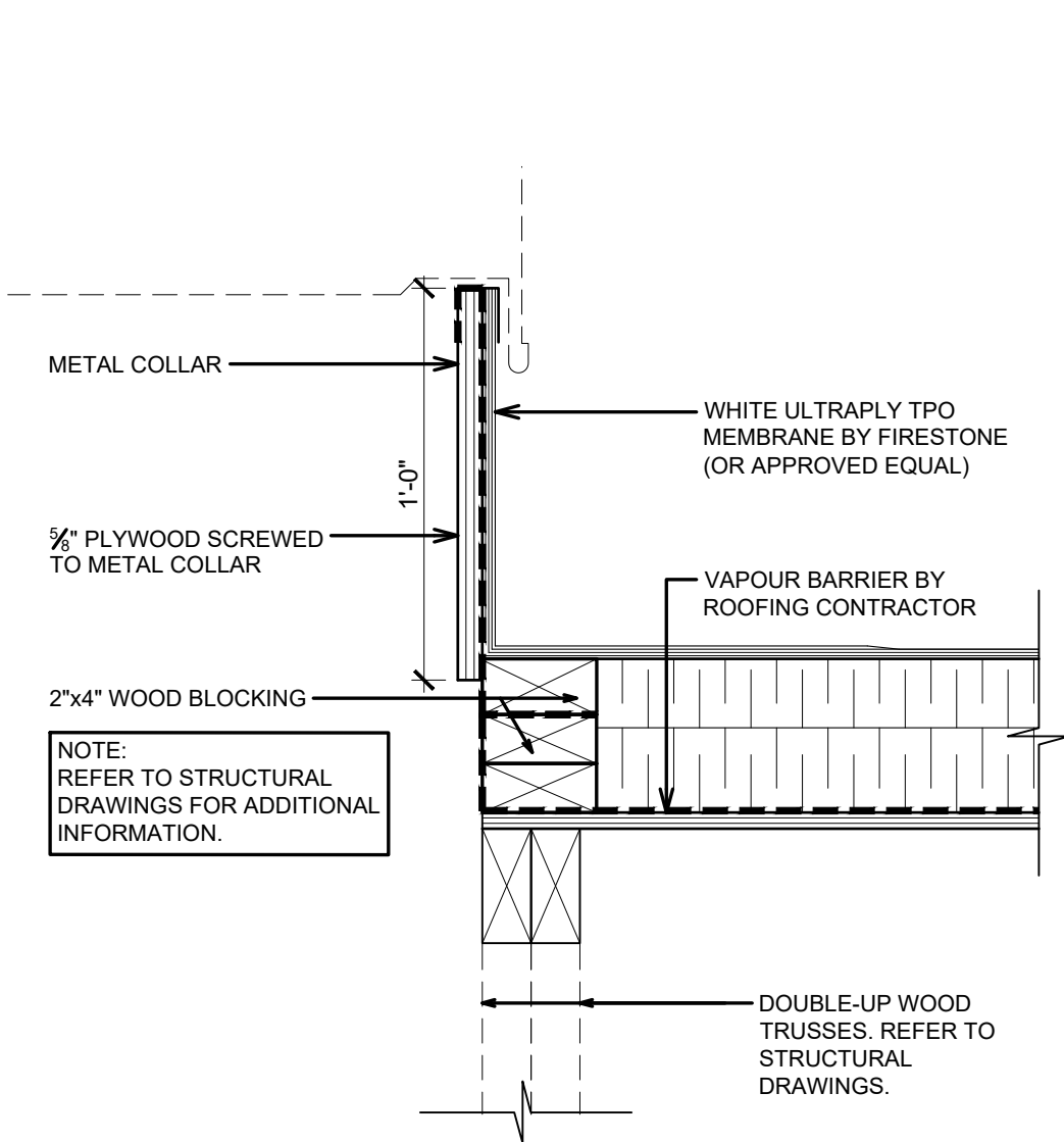
2 TYPICAL ROOF CURB DETAIL SCALE: 2"=1'-0"
