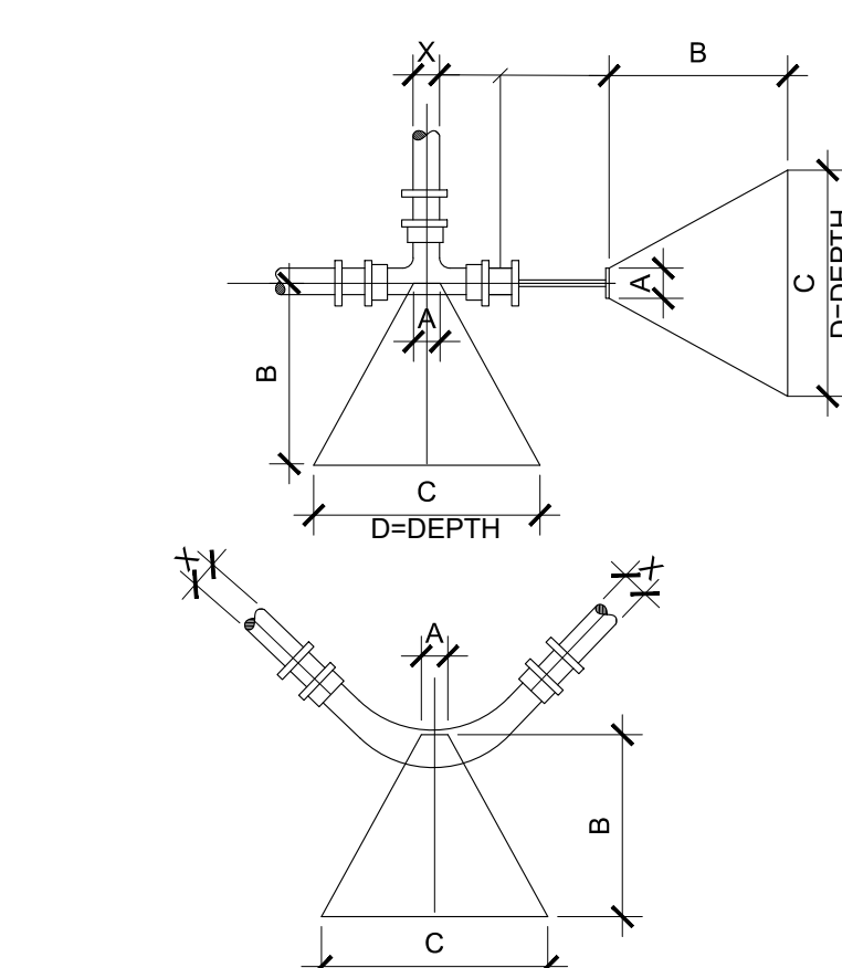
10 THRUST BLOCKS AS2.3 SCALE: 3/8" = 1'-0"
